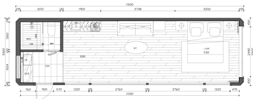
Layout plan
